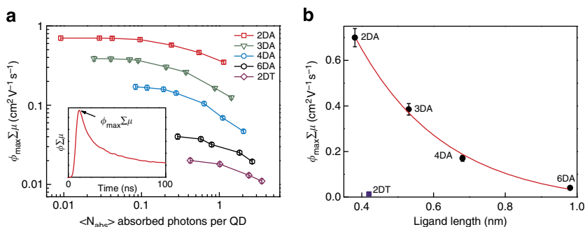
Figure 2 | Photoconductivity of the QD films. (a) \phi_{\text{max}} \Sigma \mu values as a function of the average number of absorbed photons per QD for QD films with various replacing ligands. The inset shows a typical photoconductance transient and the point that corresponds to \phi_{\text{max}} \Sigma \mu . (b) \phi_{\text{max}} \Sigma \mu values for alkyl diamine ligands with different carbon chain lengths. Note that 2DT shows a much lower \phi_{\text{max}} \Sigma \mu value than 2DA. Error bars indicate the s.d.
